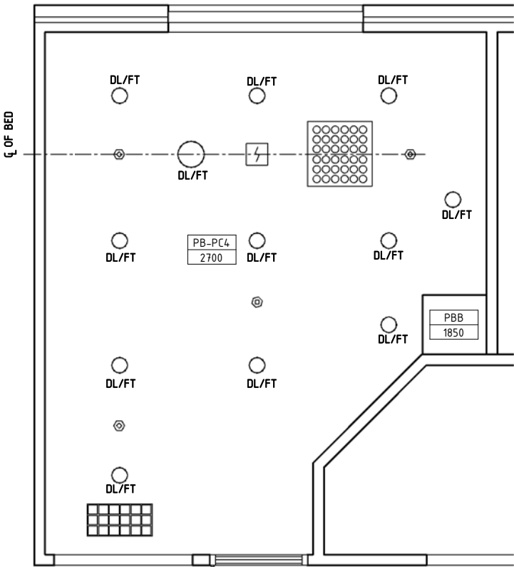
REFLECTED CEILING PLAN
