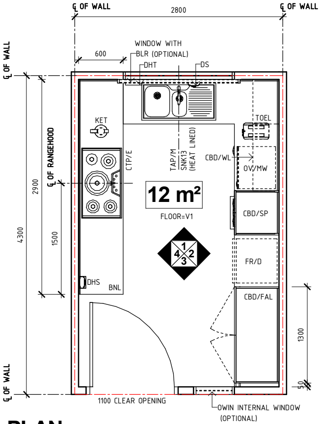
PLAN
