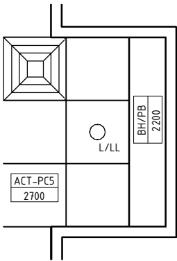
REFLECTED CEILING PLAN
