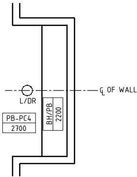
REFLECTED CEILING PLAN
