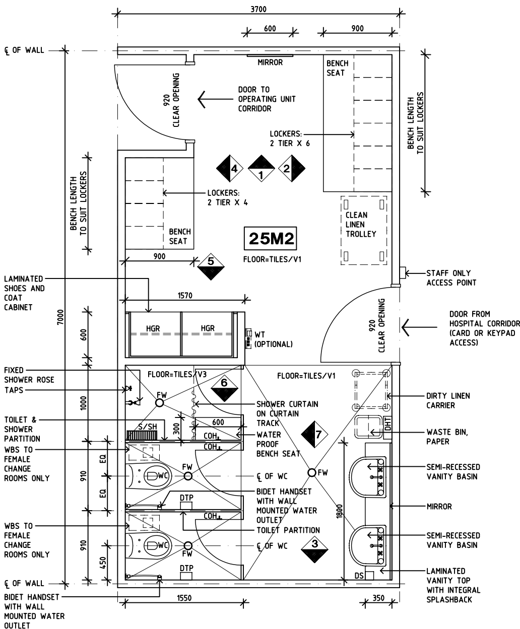
PLAN
