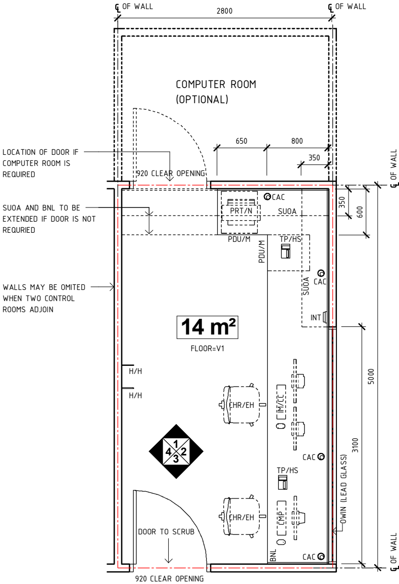
PLAN
