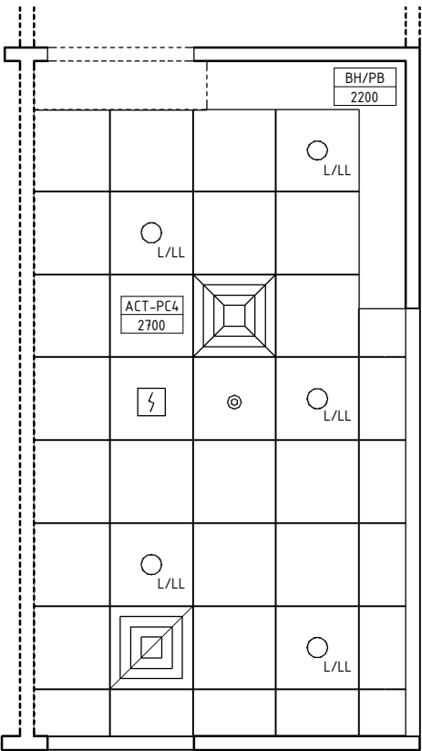
REFLECTED CEILING PLAN
