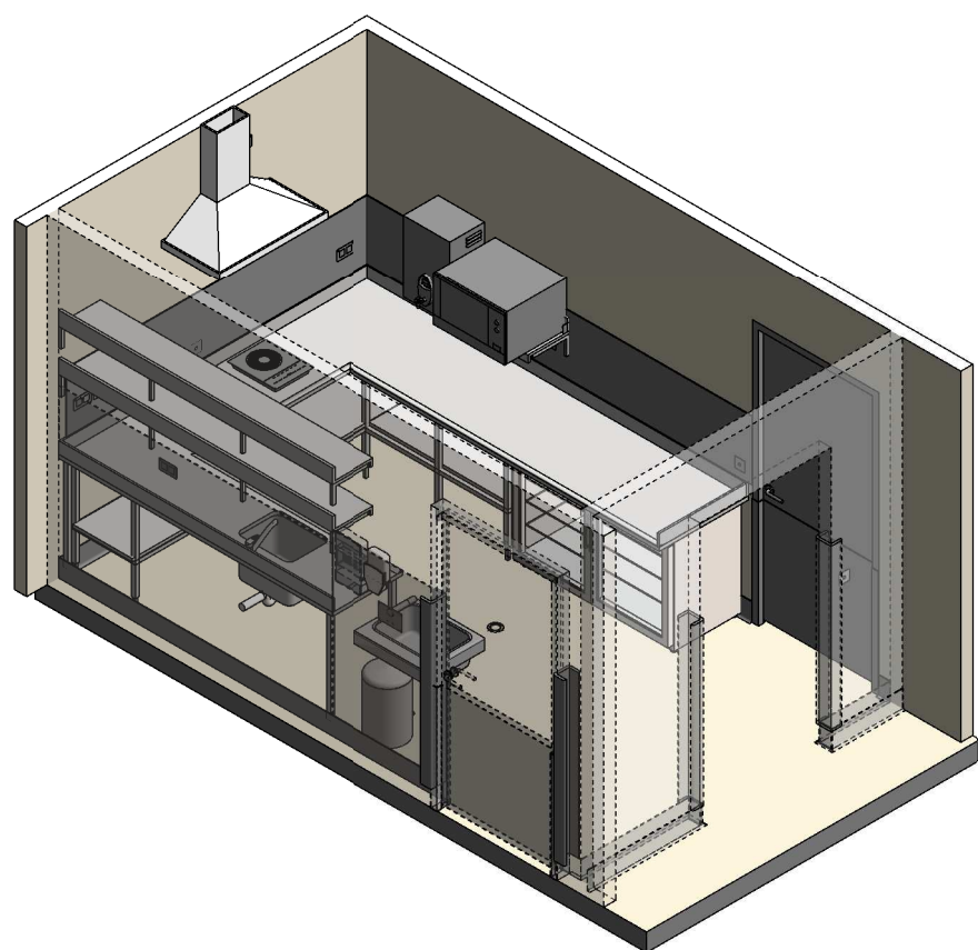
ISOMETRIC VIEW 01
