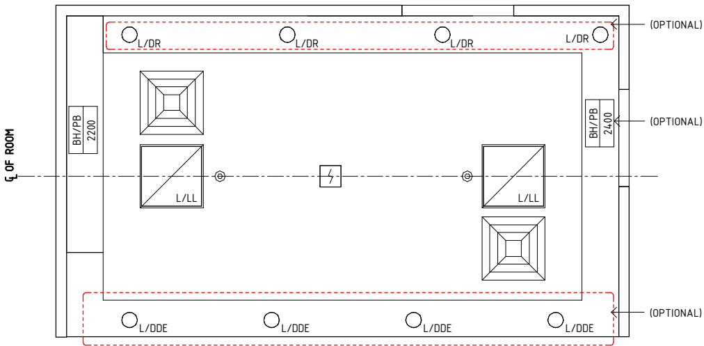
REFLECTED CEILING PLAN
