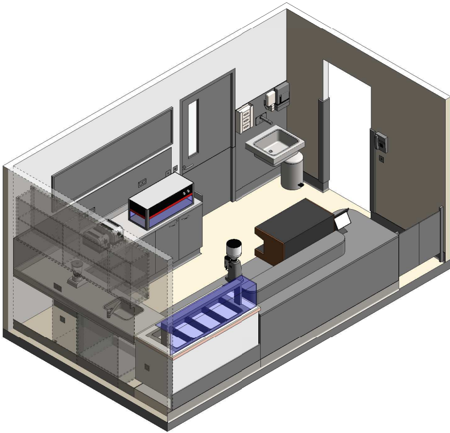
ISOMETRIC VIEW 02
