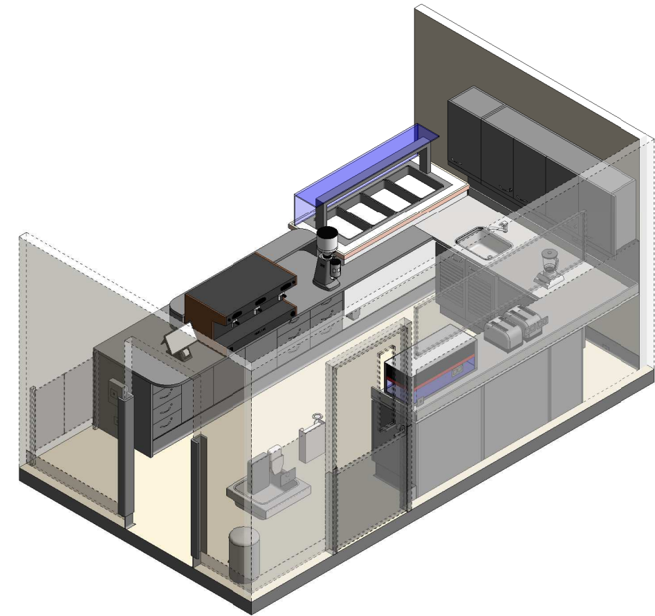
ISOMETRIC VIEW 01
