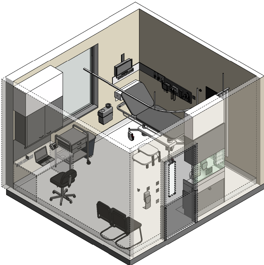
ISOMETRIC VIEW 02
