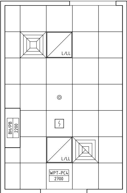
REFLECTED CEILING PLAN
