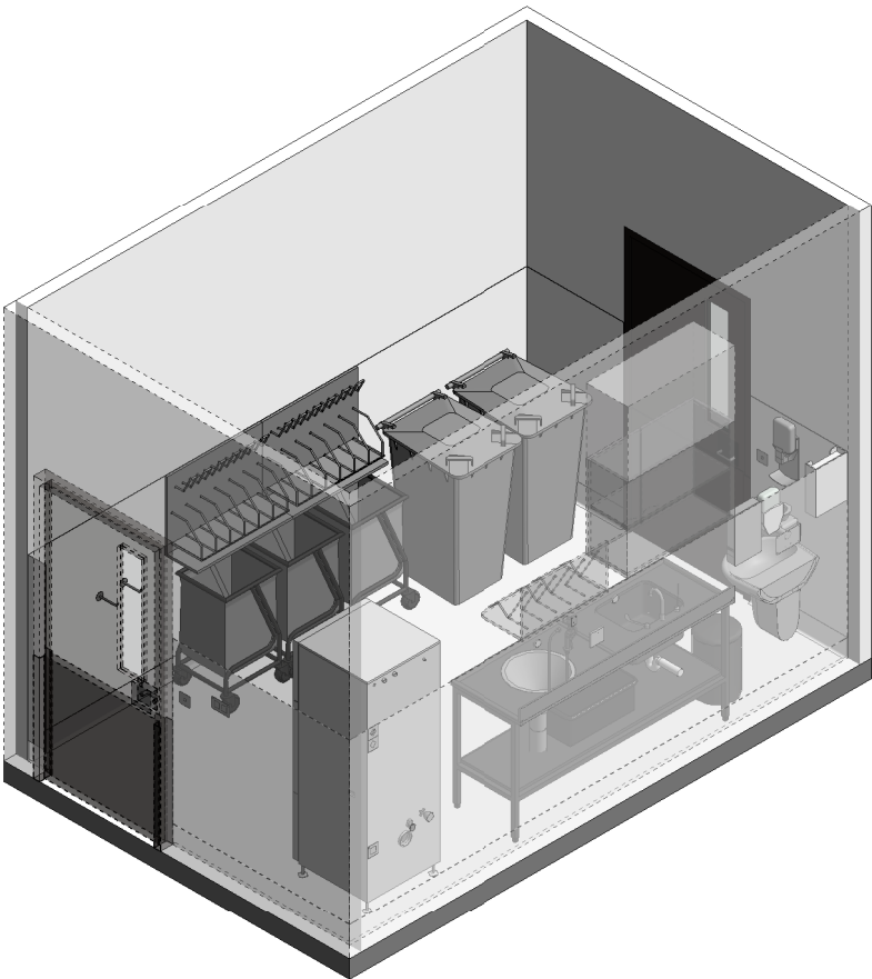
ISOMETRIC VIEW 2
