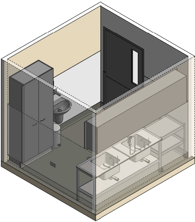
ISOMETRIC VIEW 02
