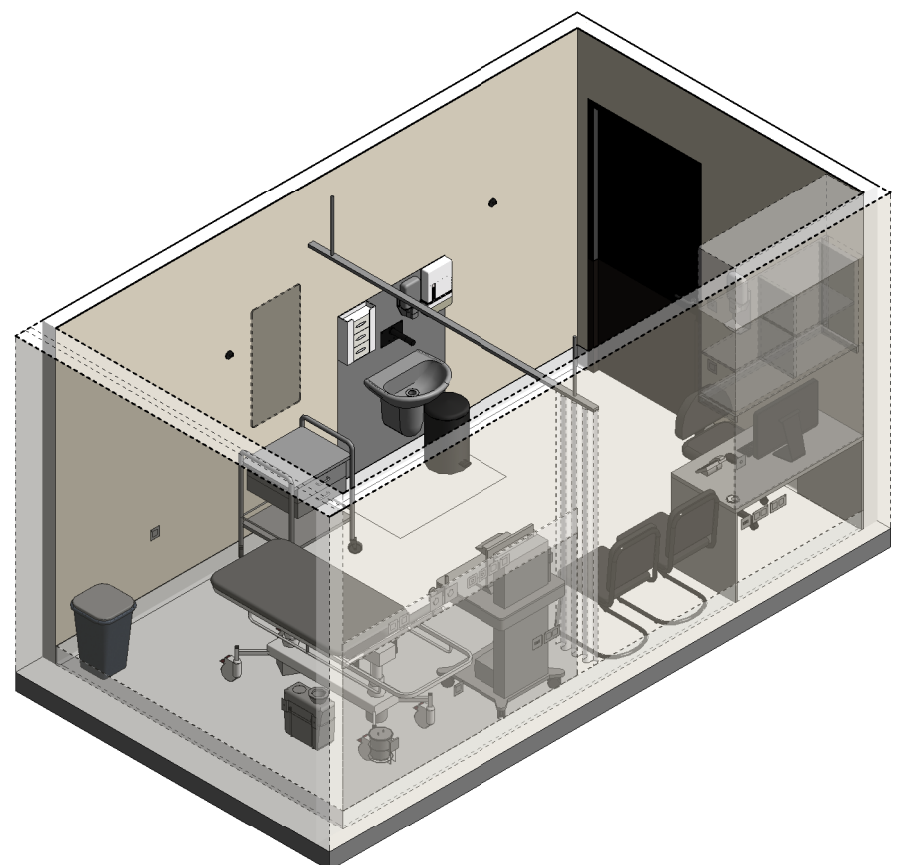
ISOMETRIC VIEW 2
