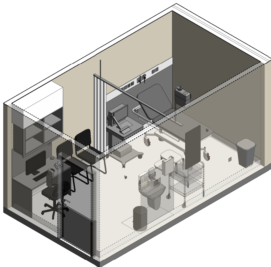
ISOMETRIC VIEW 1
