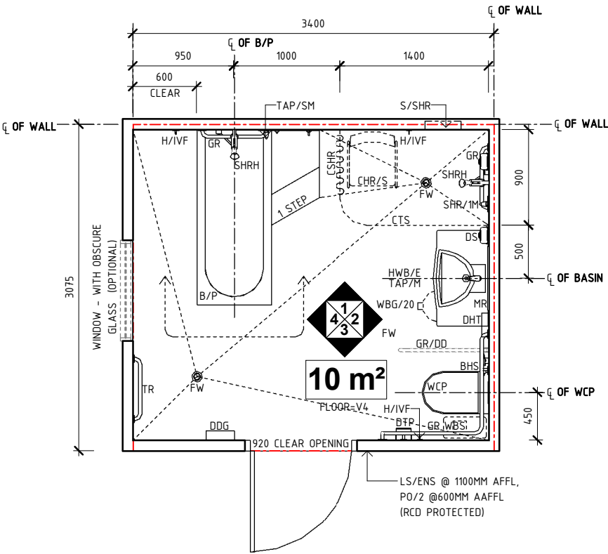
PLAN
