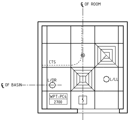
REFLECTED CEILING PLAN
