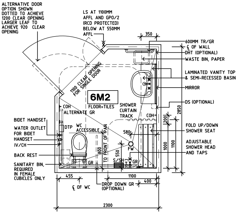
PLAN
