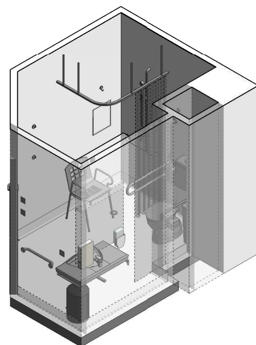
ISOMETRIC VIEW 2
