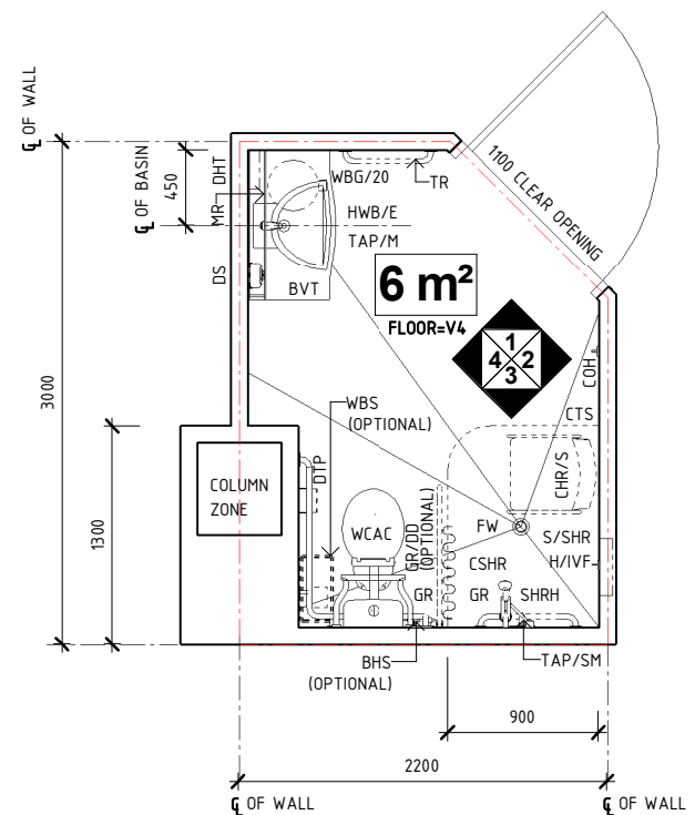
PLAN
