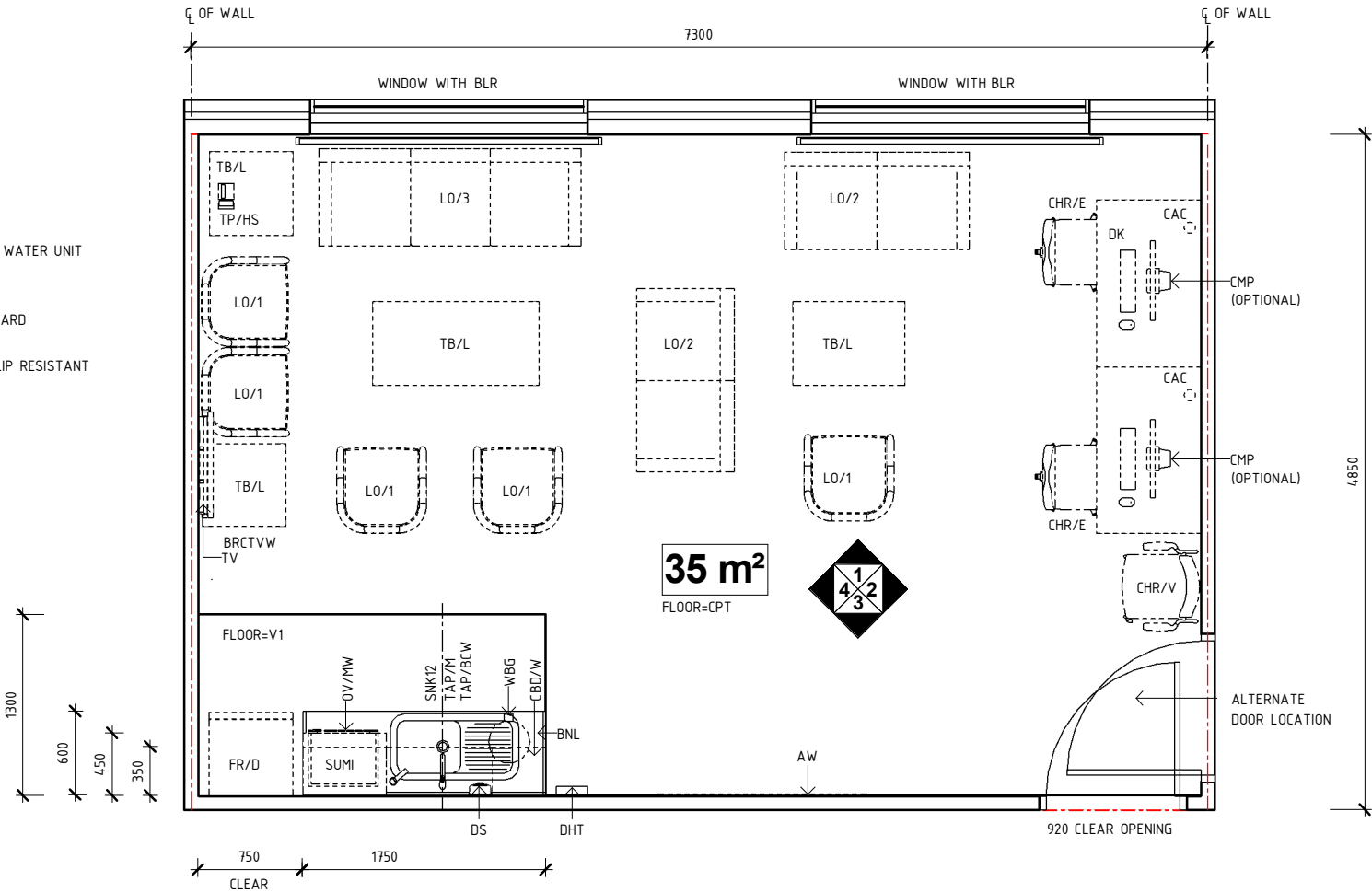
PLAN
