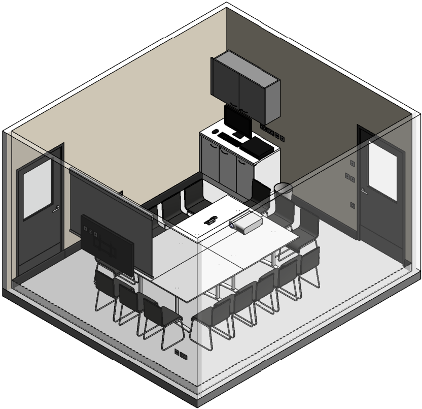
ISOMETRIC VIEW 01
