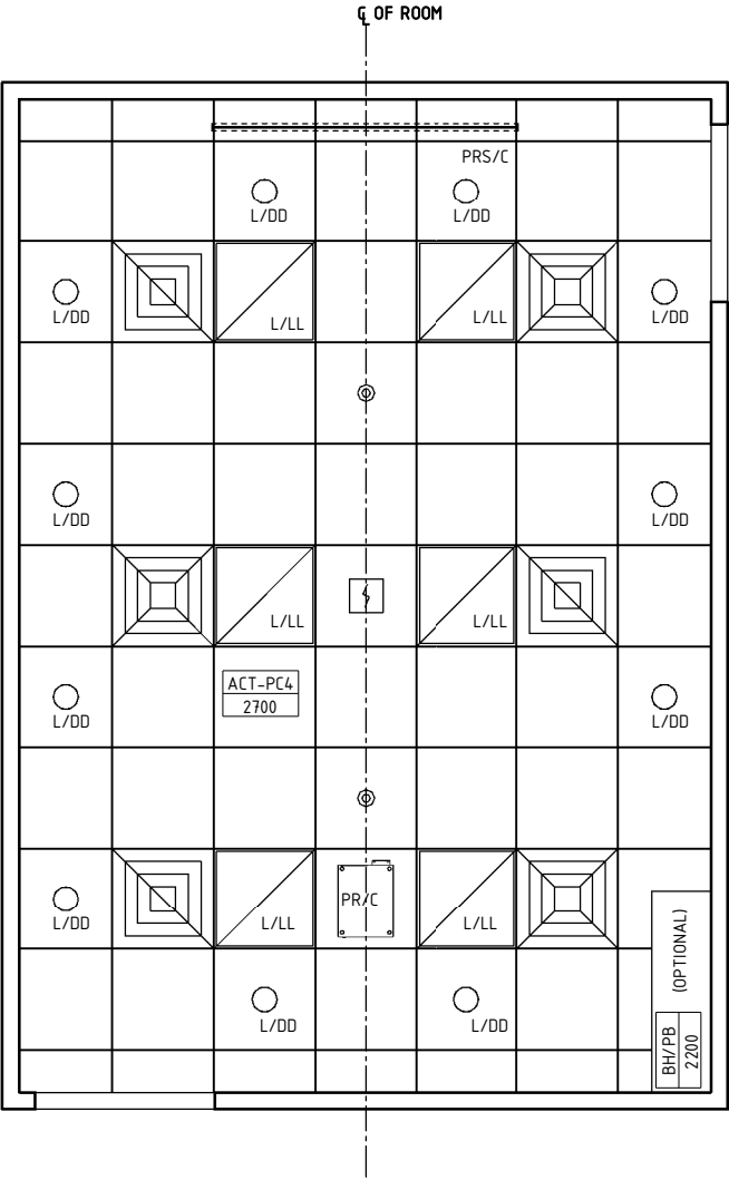
REFLECTED CEILING PLAN
