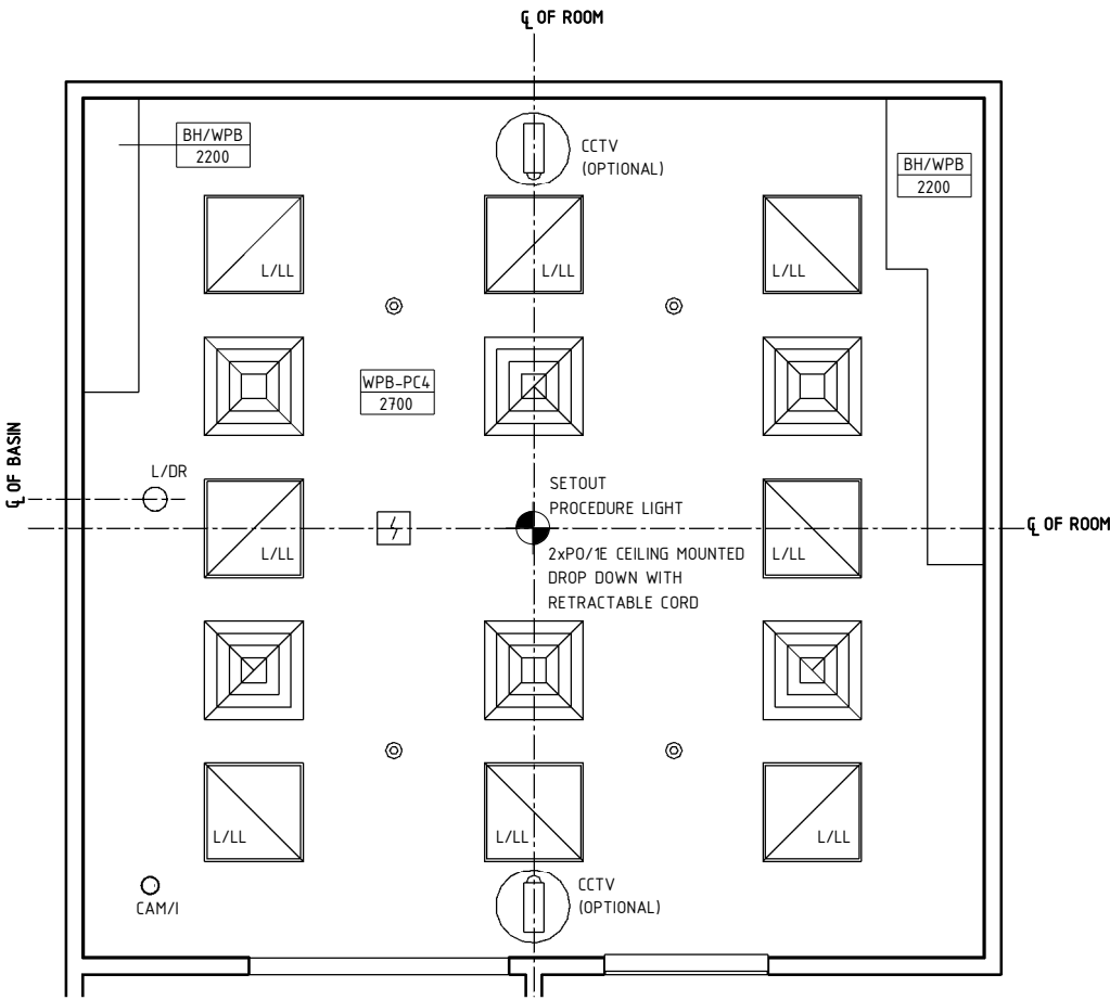
REFLECTED CEILING PLAN
