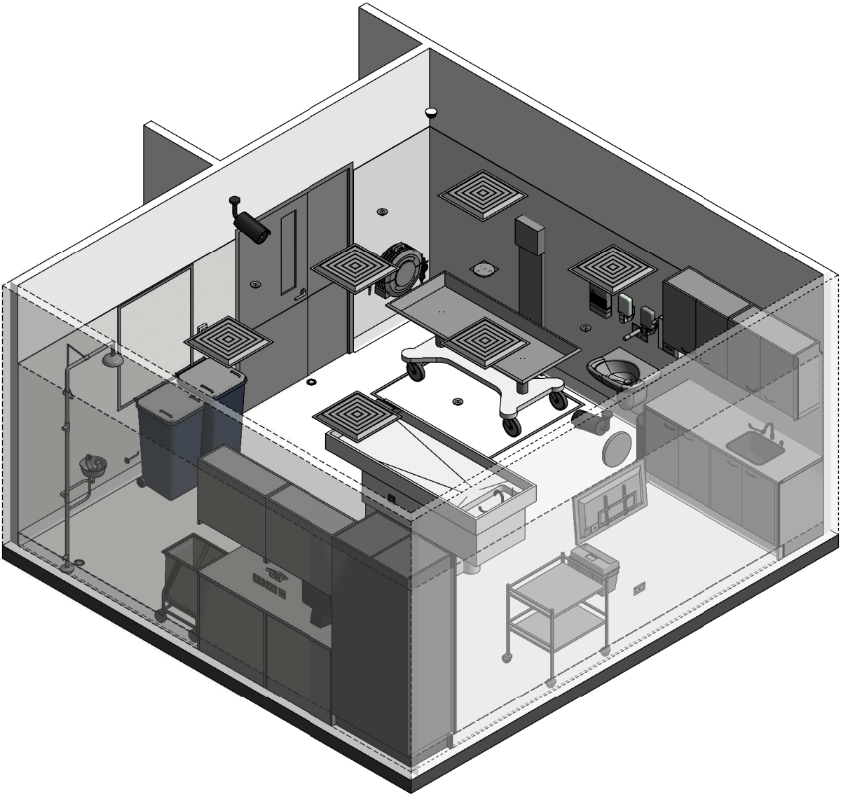
ISOMETRIC VIEW 01
