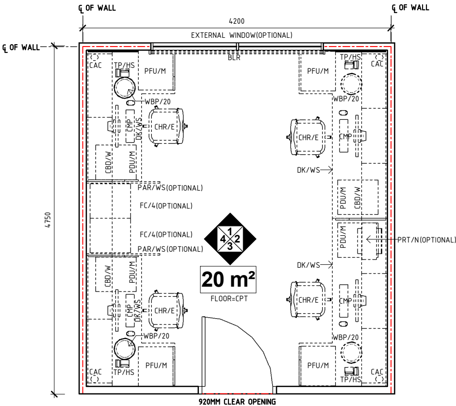
PLAN
