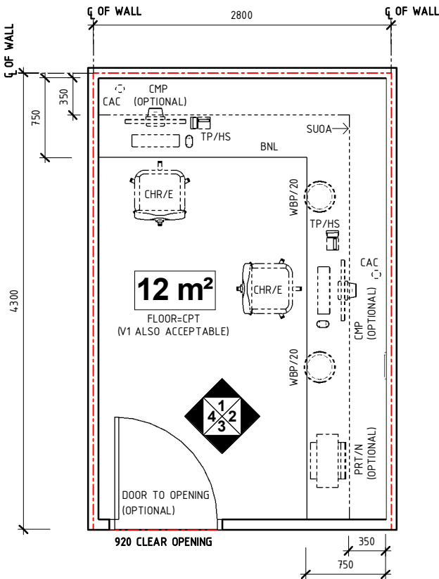
PLAN
