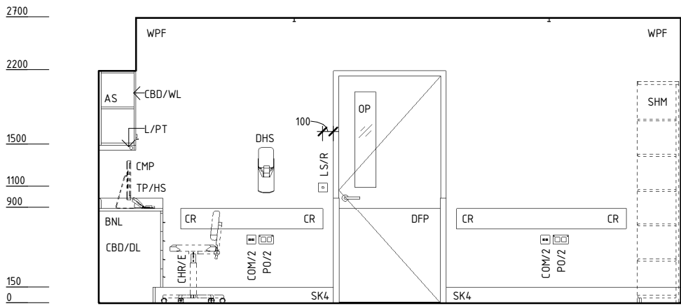
ELEVATION 03
