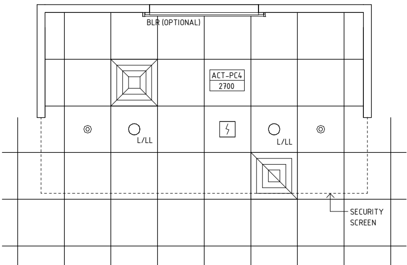
REFLECTED CEILING PLAN
