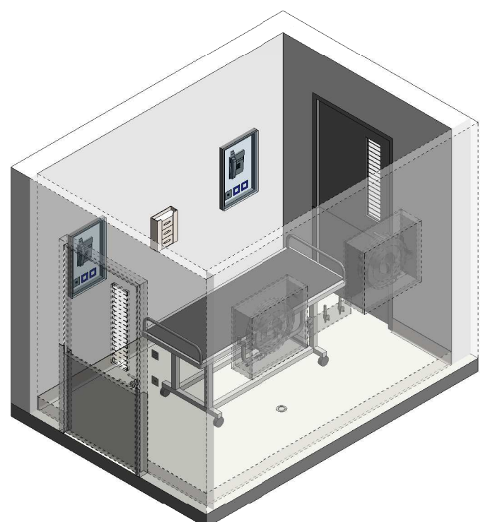
ISOMETRIC VIEW 02
