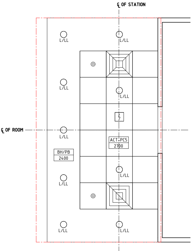
REFLECTED CEILING PLAN
