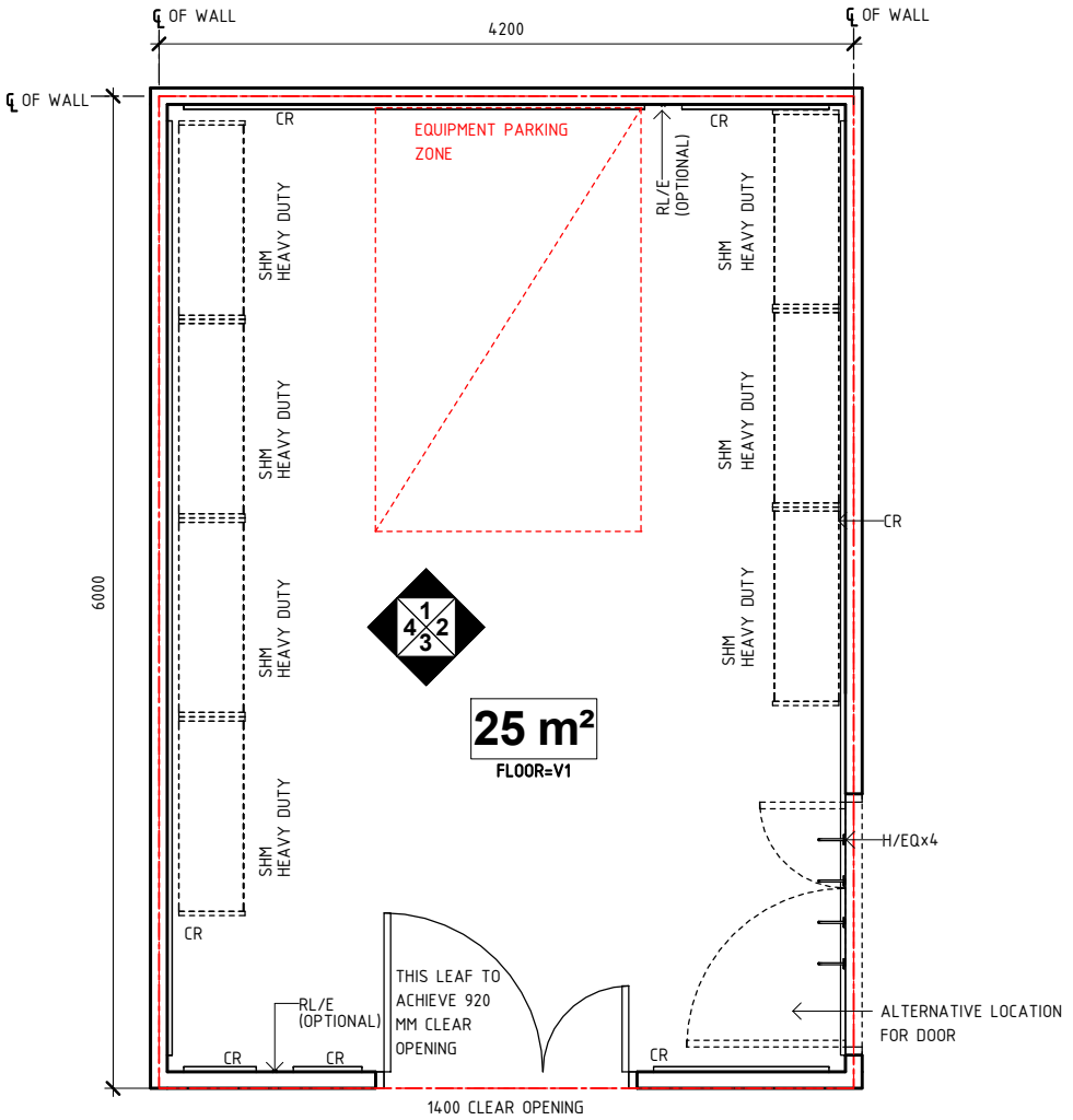
PLAN
