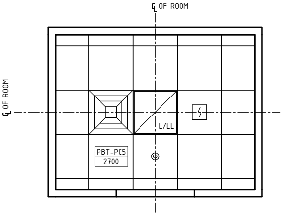
REFLECTED CEILING PLAN
