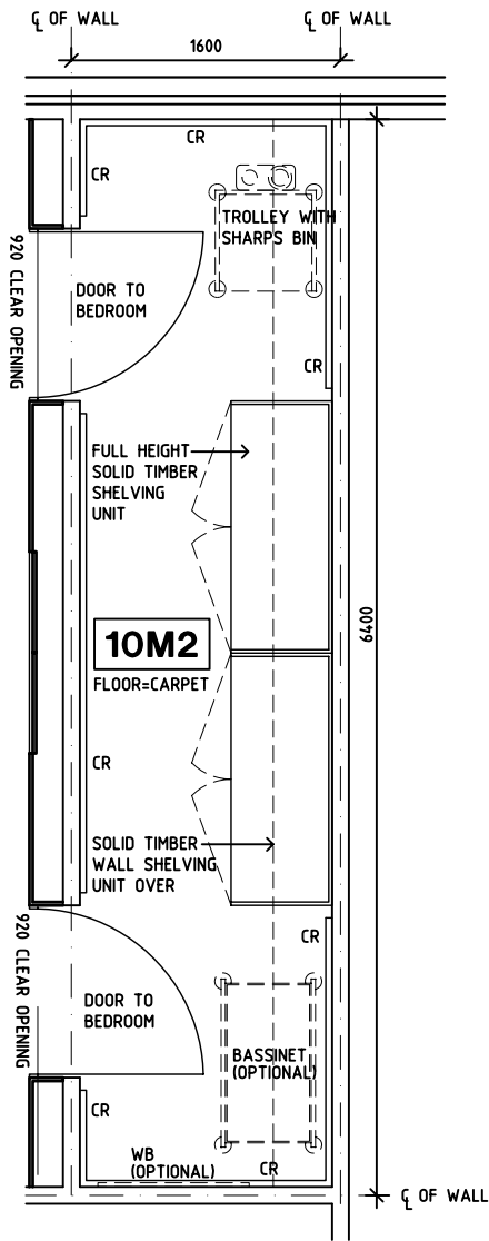
PLAN
