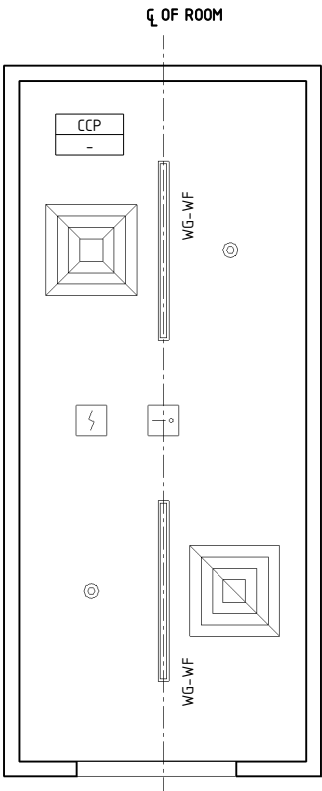
REFLECTED CEILING PLAN
