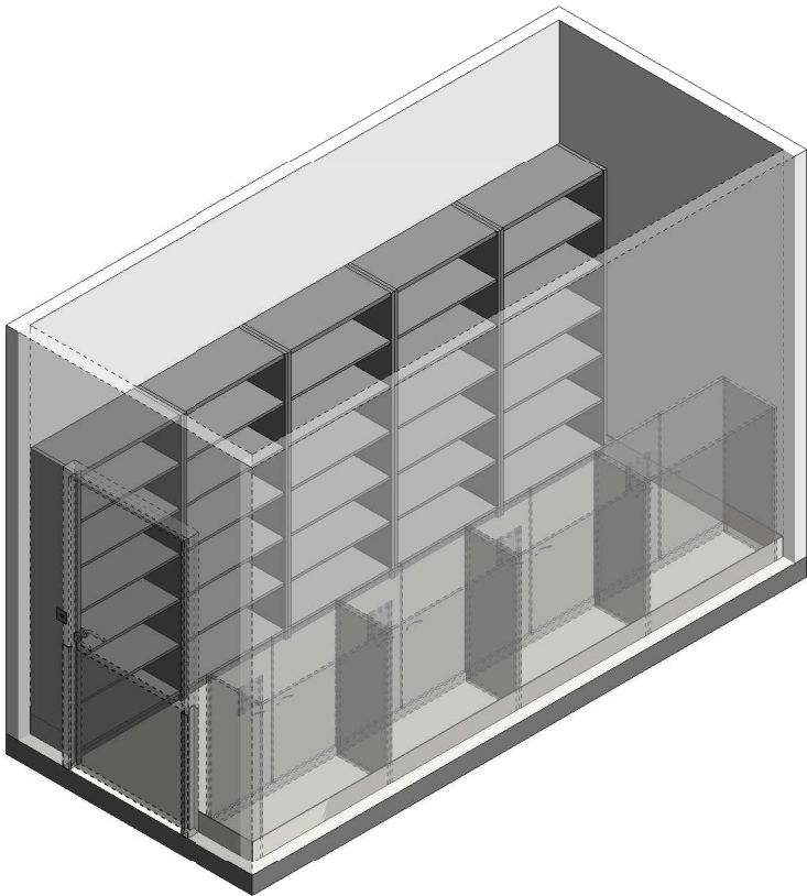
ISOMETRIC VIEW 01
