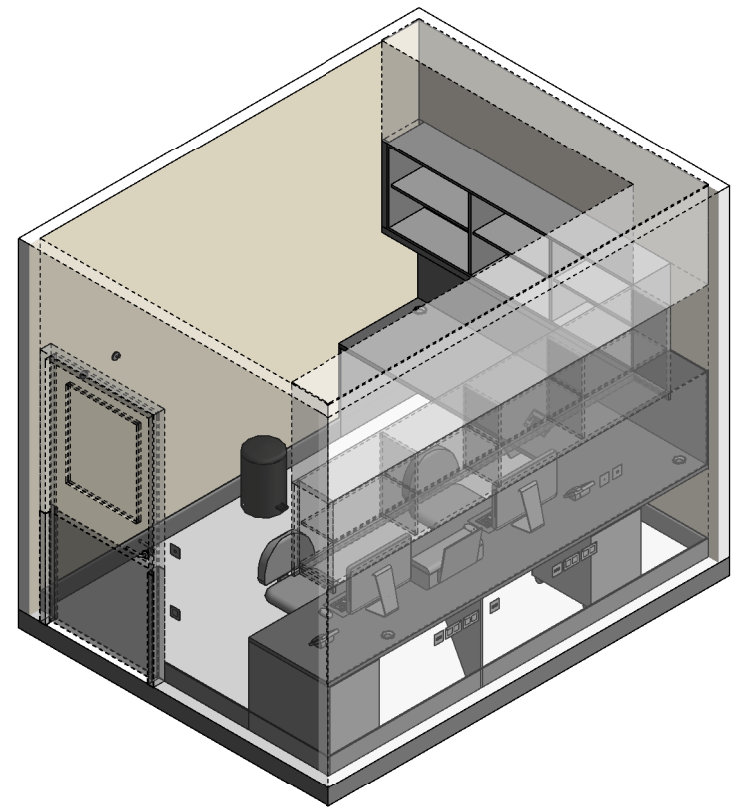
ISOMETRIC VIEW 01
