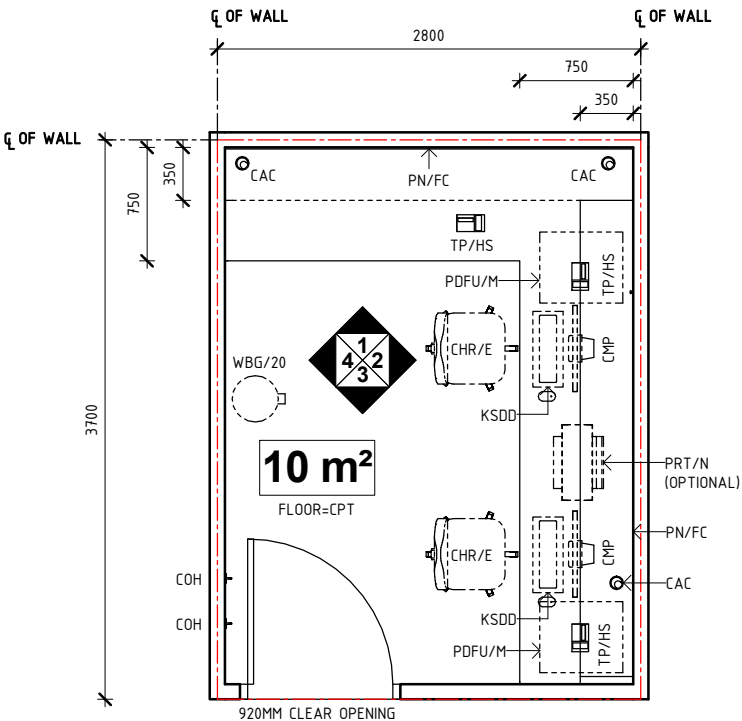
PLAN
