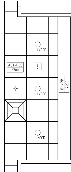
REFLECTED CEILING PLAN
