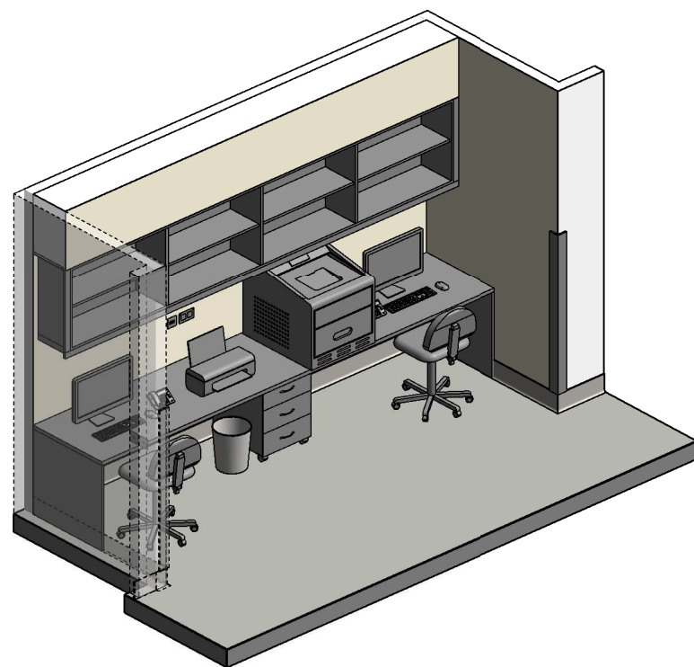
ISOMETRIC VIEW 01
