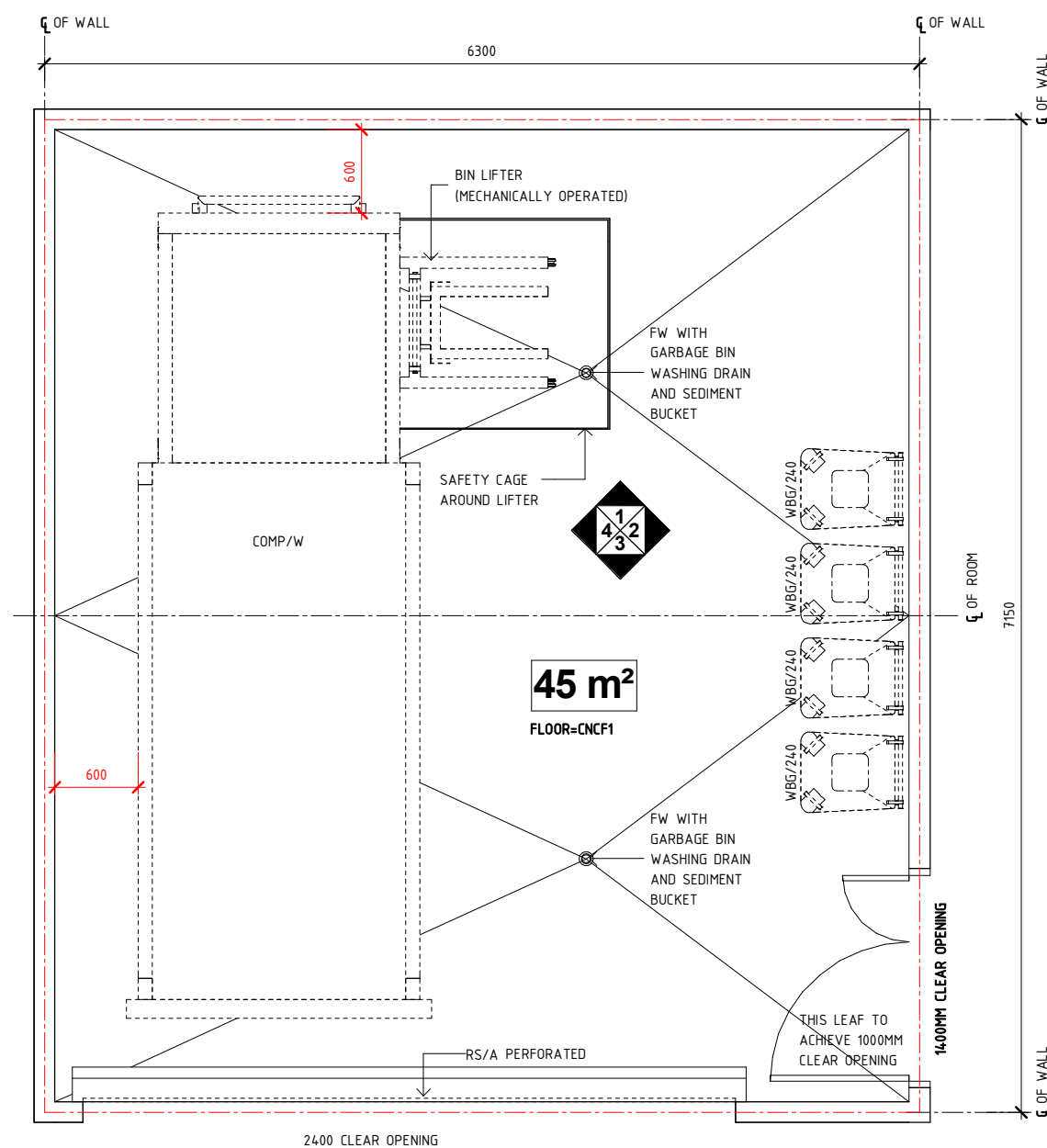
PLAN
