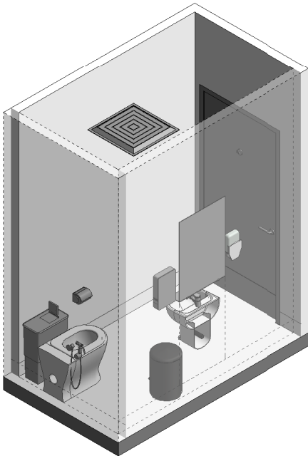
ISOMETRIC VIEW 02
